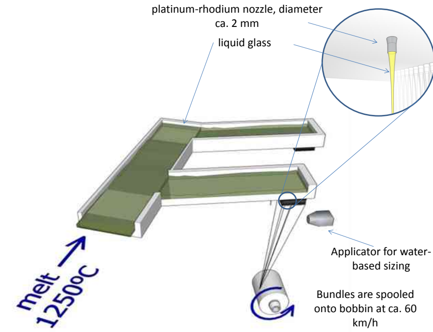
Figure 4: Overview of glass fibre production
