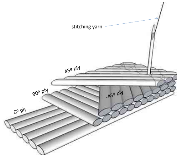
Figure 10: Production of a quasi-isotropic non-crimp fabric by stitching (based on [7])
