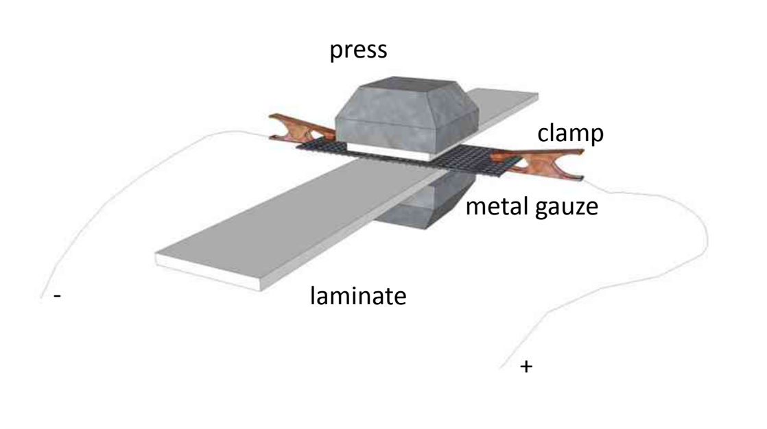
Figure 55: Welding of thermoplastics (based on [4])
